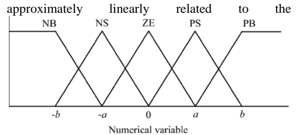
Fig. 3. Membership function for inputs and output of fuzzy logic controller.
