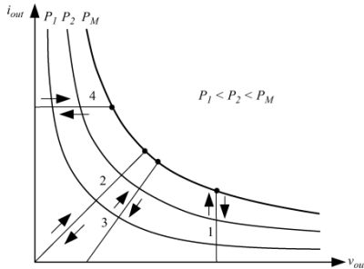
Fig. 7. Different load types. 1: voltage source, 2: resistive, 3: resistive and voltage source, 4: current source, as shown in [78].
