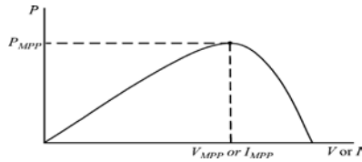
Fig. 1. Characteristic PV array power curve.
