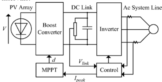
Fig. 5. Topology for dc-link capacitor droop control as shown in [71].
