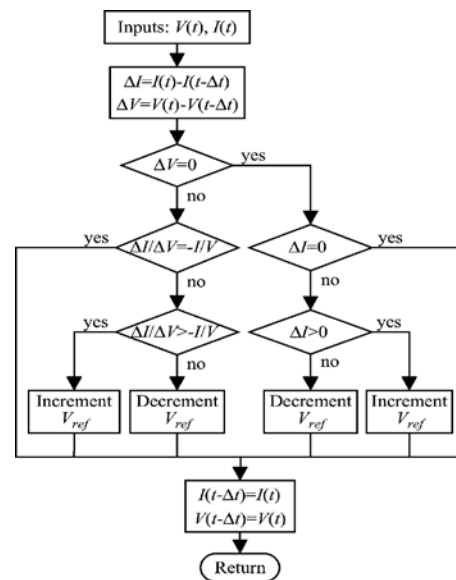
Fig. 2. IncCond algorithm chart.
