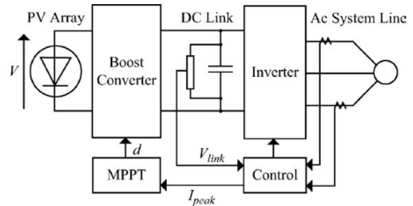
Fig. 6. Topology for dc-link capacitor droop control as shown in [71].
