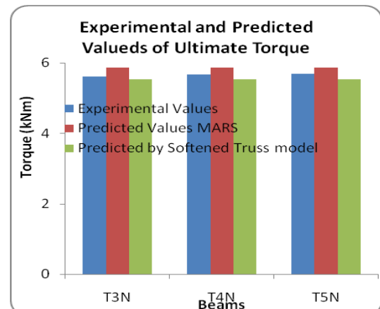
Fig.3 Torque variation of only Transverse reinforced beams
