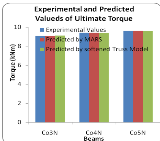
Fig.6 Experimental and Predicted Torque of over reinforced beams for different layers
