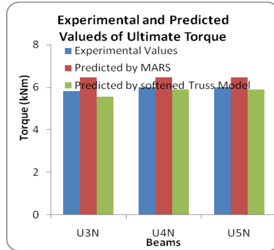
Fig.4 Experimental and Predicted values of Torque for under reinforced beams
