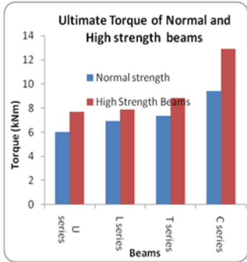
Fig.8 Comparison of Torque between normal strength and high strength Beams for 4 layers
