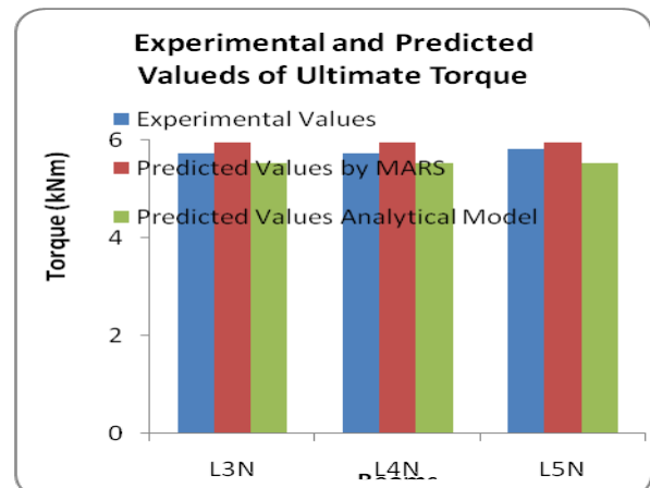
Fig.2 Variation of torque of only longitudinally reinforced beams
