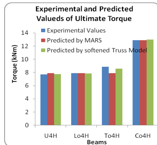
Fig.7 Comparison of Torque between Experimental and Predicted Values for high strength Beams for different states of Torsion
