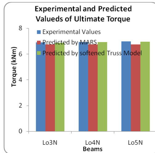
Fig.5 Experimental and Predicted Torque variation of longitudinally over reinforced beams
