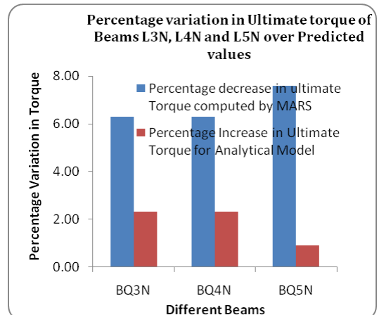
Fig.1 Percentage Variation in Ultimate Torque of predicted by analytical model and MARS over Experimental Values
