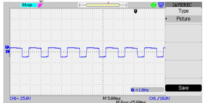
Fig.16: Output of Schmitt Trigger
