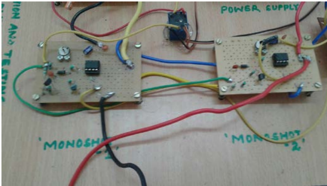
Fig.18: Hardware fabricated Monoshot multivibrator1 &2
