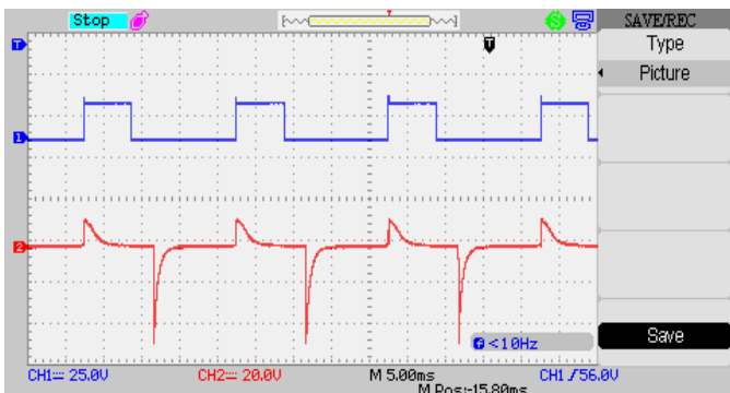
Fig.19:Output of Monoshot Multivibrator 1
