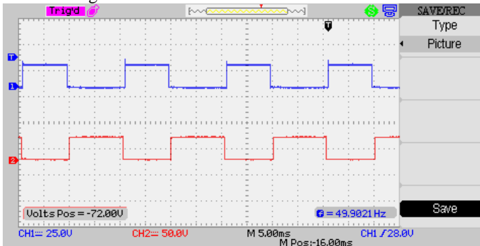
Fig.20: Output of Monoshot Multivibrator 1 and 2
