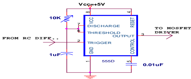
Fig 6: Monoshot Multivibrator
