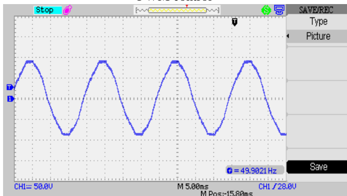
Fig.25: Oscilloscopic traces of UPS with using a PWM control
