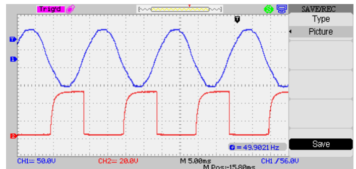
Fig.22: Output of ZCD
