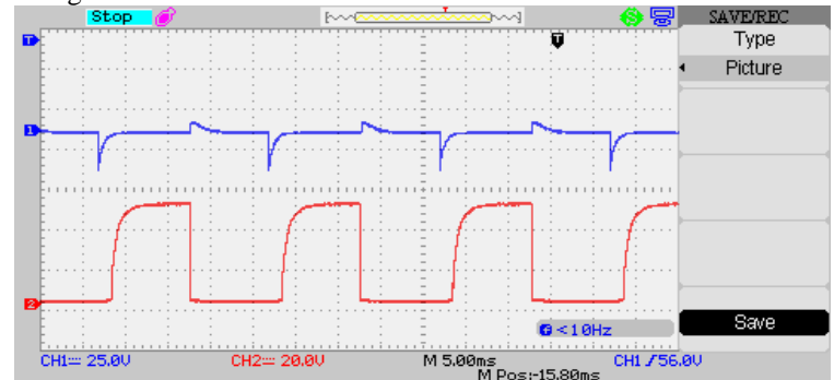
Fig.21: Output of RC Differentiator and ZCD
