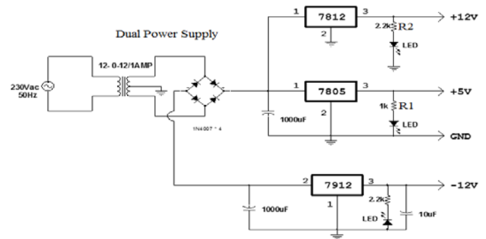
Fig.2: Dual Power Supply
