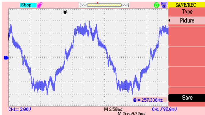
Fig.24: Oscilloscopic traces of UPS without using a PWM control
