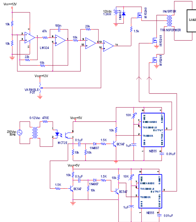
Fig.1: UPS Using PWM
