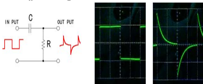
Fig.7: RC Differentiator with their waveform
