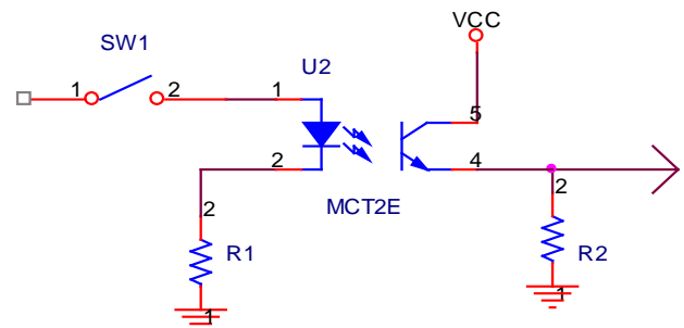
Fig.9: Circuit connection of Opto coupler
