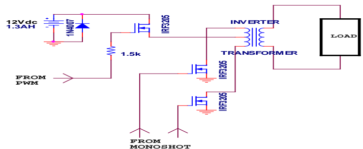
Fig.4: Circuit Diagram of PWM Converter
