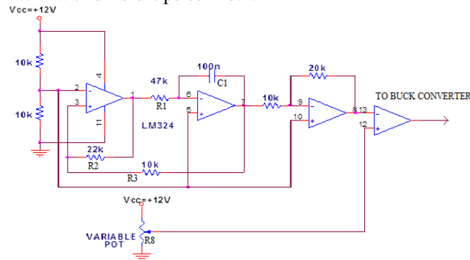
Fig.3: Schematic diagram of PWM Generator
