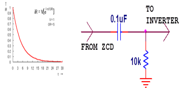
Fig.8: (a) iR drop vs time and (b) designed components in RC differentiator
