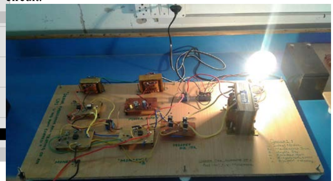
Fig.23: Hardware fabricated UPS circuit
