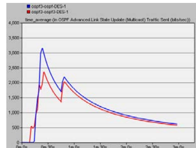
Fig. 3 Link State Update (Multicast) traffic sent
