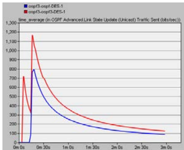
Fig. 4 Link State Update (Unicast) traffic sent
