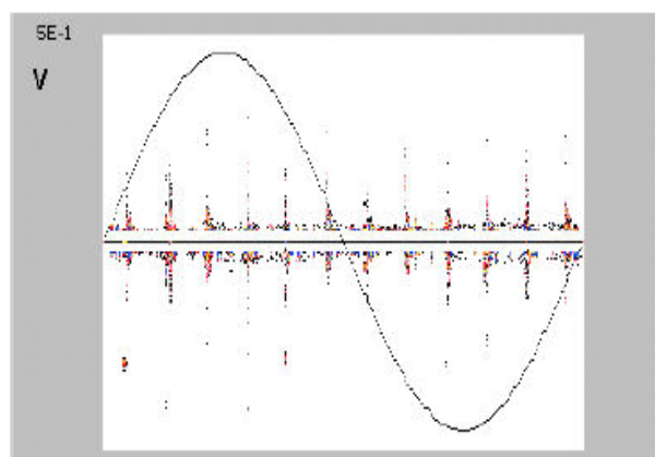
Figure 2 - Phase-resolved PD measurement of repetitive switching noise of the 12-pulse HVDC converter [4]
