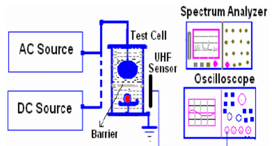
Figure 4- PD measurement setup based on UHF signal detection [4]
