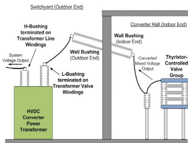
Figure 1- HVDC station equipment arrangement [3]
