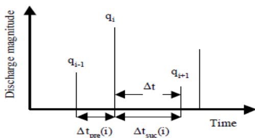
Figure 3 – PD signals due to HVDC stress [7]
