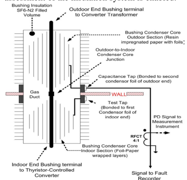
Figure 5 - HVDC wall-bushing on-line PD measurement[3]
