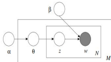
Fig. 1 LDA Graphical representation
