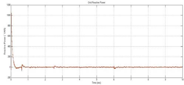
Fig. 14. Grid reactive power
