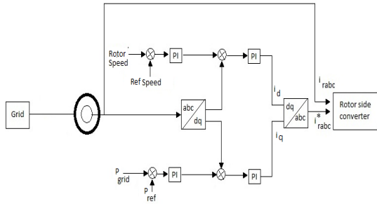
Fig .5.Control of Rotor Side Converter
