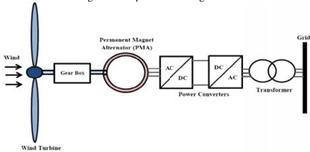
Fig.2. Synchronous generator with full converter
