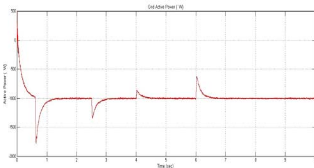
Fig. 13. Grid power variations with respect to time
