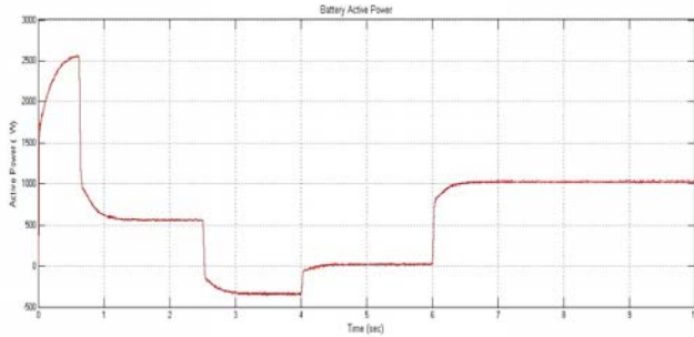
Fig. 12. Active power supplied by the stator of the BESS
