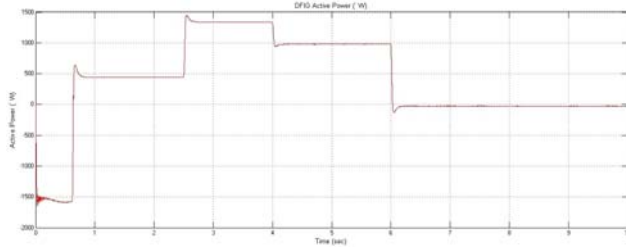
Fig. 11. Active power supplied by the stator of the DFIG
