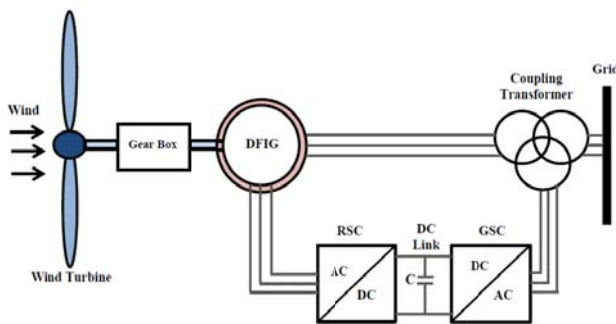
Fig.3. Doubly fed induction generator
