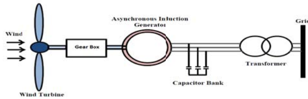
Fig.1. Fixed speed induction generator
