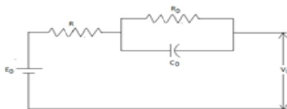
Fig.8.. Battery model
