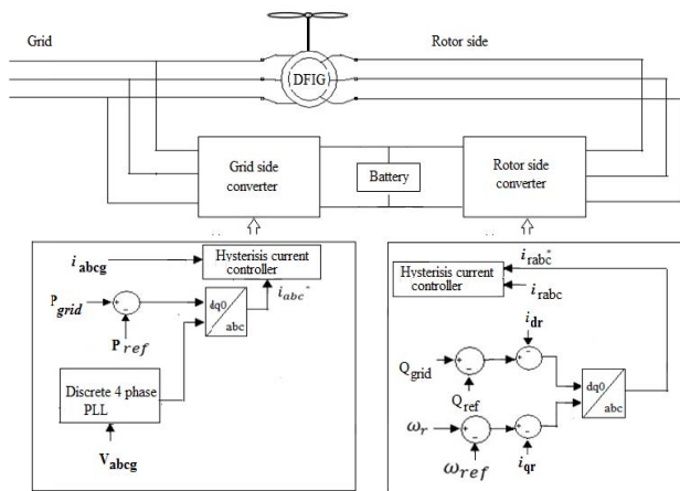
Fig.4. DFIG control scheme
